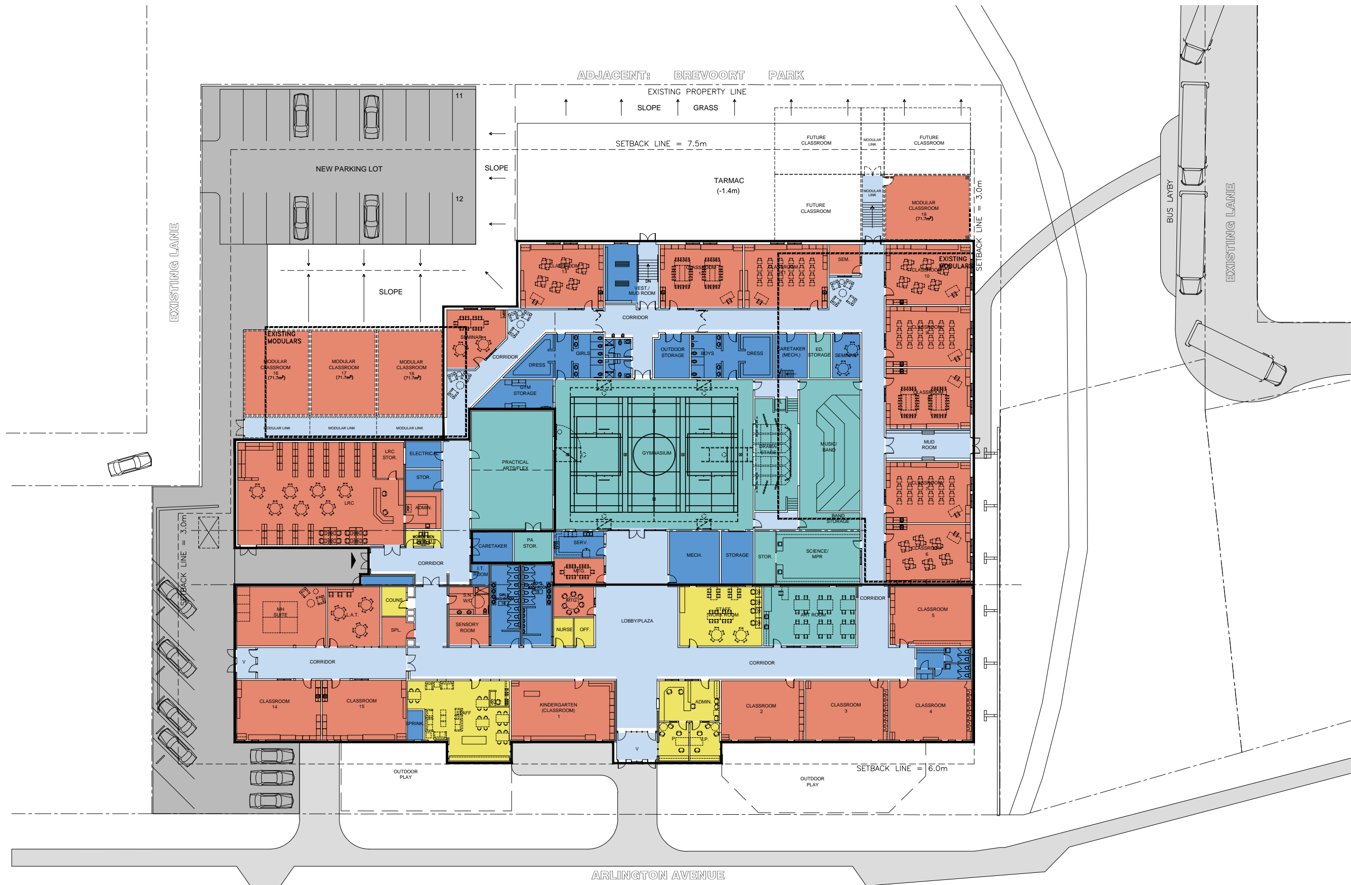
NORTH 1 MAIN FLOOR PLAN SCALE 1:200
