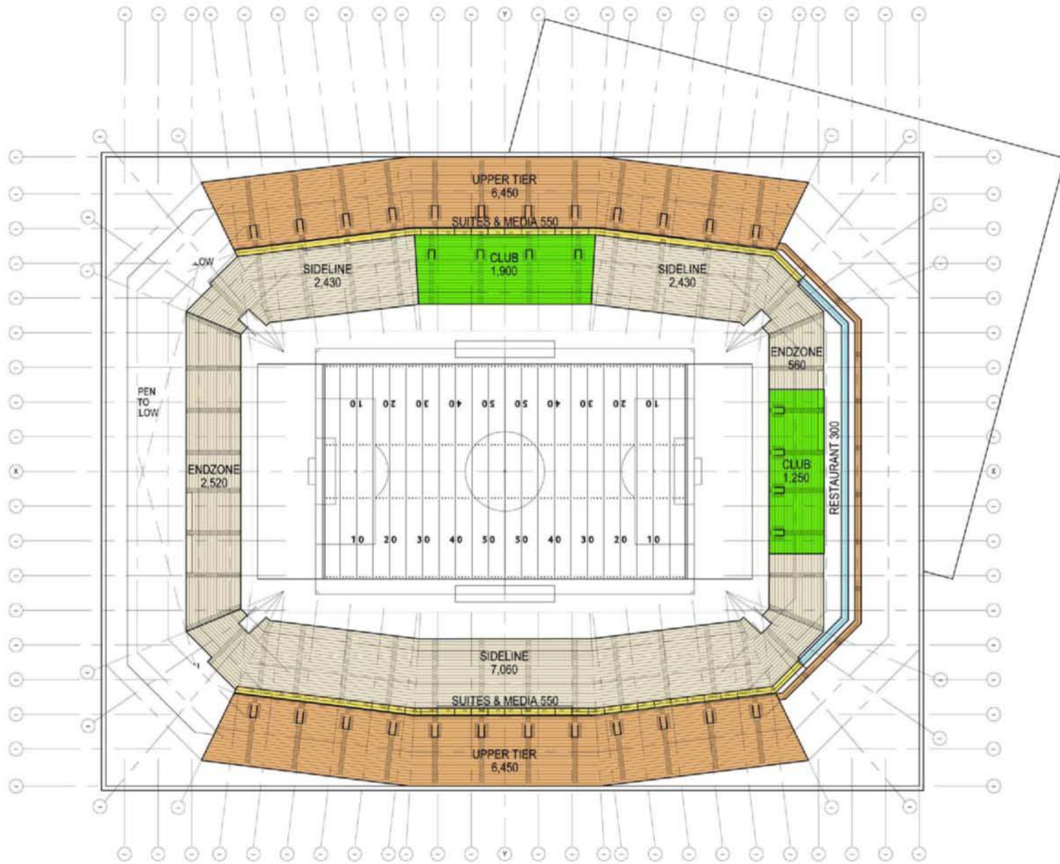
Seating Bowl Plan – 33,000 Spectators
